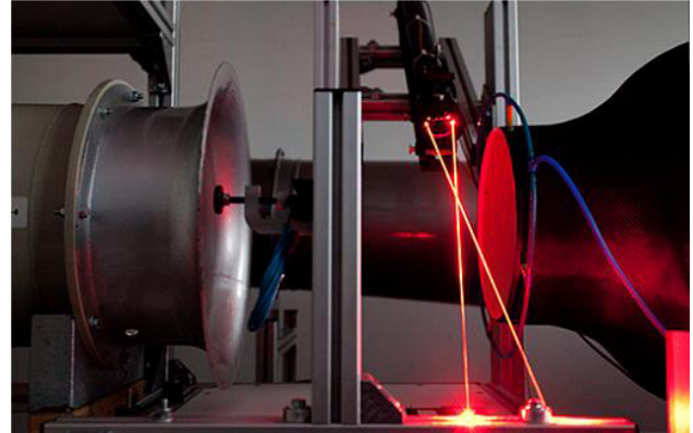
Fig. 1: Calibration of wind tunnel with HeNe-based LDV-System at Westenberg Engineering
